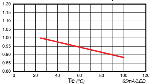
Relative Luminous Flux / Tc Temperature
