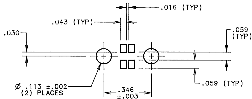
SOLDER PAD AND HOLES LAYOUT
